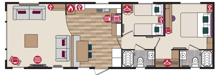
42ft x 14ft - 2 bedroom
